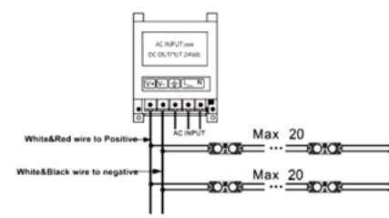
WIRE CONNECTION
