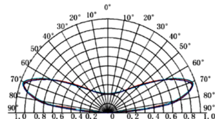
BEAMING ANGLE
